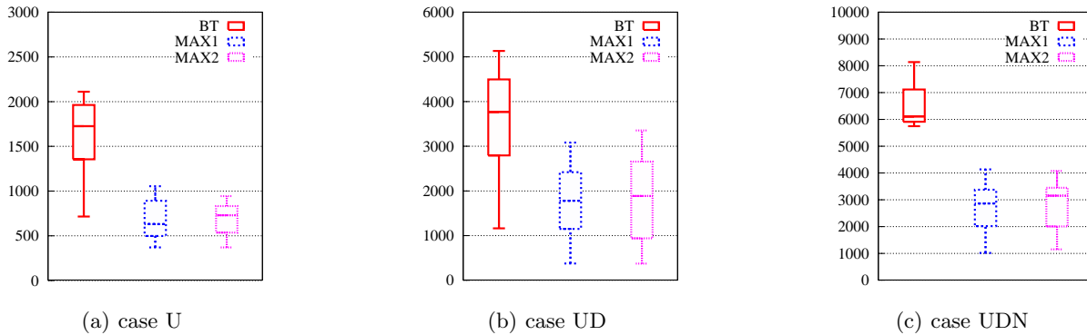
Figure 4: A comprehensive overview of results: Boxplot of download times when more and more stringent bottlenecks are introduced in experiments ( n=100 peers, FS = 500 MB, for case UDN there is a 2 Mbps network bottleneck). The two BitMax algorithms maintain their gain in performance over BT across all scenarios, and they are less sensitive to severe network conditions. Note the different scale of the boxplots: whereas BitMax remains superior to BT in all the scenario we considered, downlink and network bottlenecks increase the time it takes to distribute the content to all peers.
